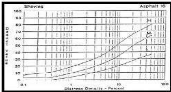
Gambar 2.41 Deduct value sungkur. (Sumber : Shahin, 1994)
