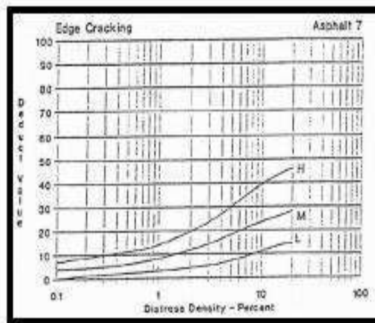
Gambar 2.28 Deduct value retak samping jalan. (Sumber : Shahin, 1994)
