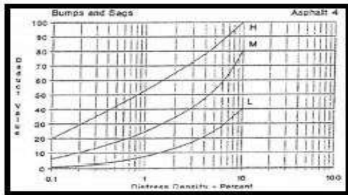
Gambar 2.26 Deduct value cekungan. (Sumber : Shahin, 1994)
