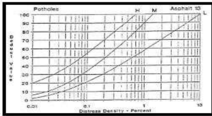
Gambar 2.35 Deduct value lubang. (Sumber : Shahin, 1994)
