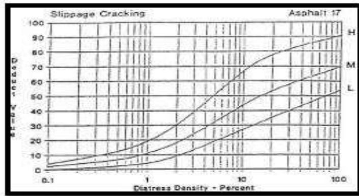
Gambar 2.36 Deduct value retak bulan sabit. (Sumber : Shahin, 1994)
