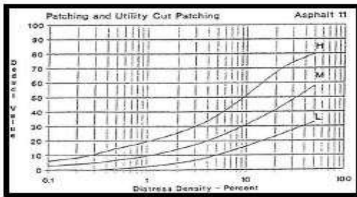
Gambar 2.33 Deduct value tambalan. (Sumber : Shahin, 1994)
