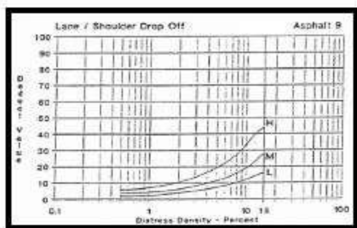
Gambar 2.31 Deduct value penurunan bahu jalan. (Sumber : Shahin, 1994)
