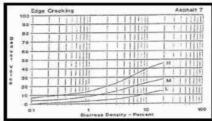
Gambar 2.29 Deduct value retak samping jalan. (Sumber : Shahin, 1994)
