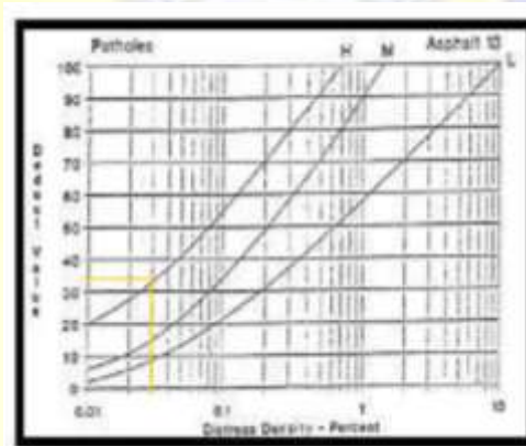
Gambar 2.34 Deduct value lubang. (Sumber : Shahin, 1994)
