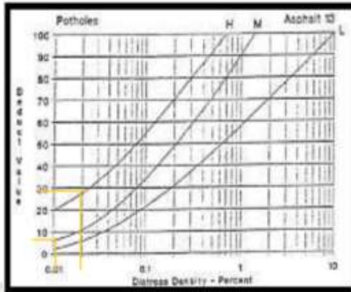
Gambar 2.34 Deduct value lubang. (Sumber : Shahin, 1994)
