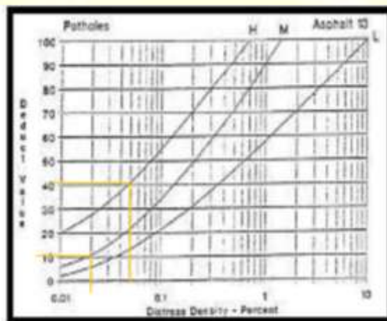
Gambar 2.34 Deduct value lubang. (Sumber : Shahin, 1994)
