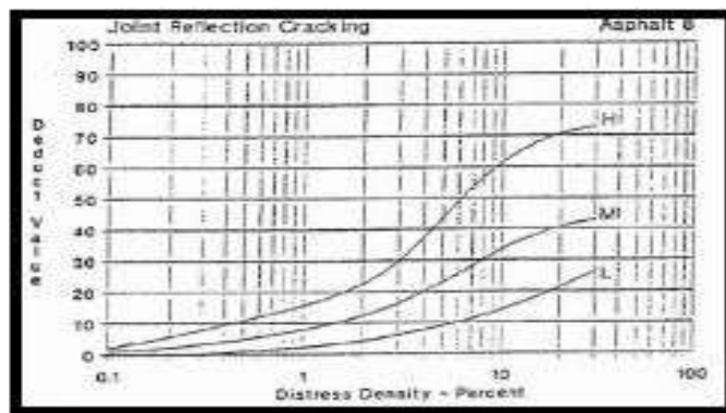
Gambar 2.30 Deduct value retak sambung. (Sumber : Shahin, 1994)
