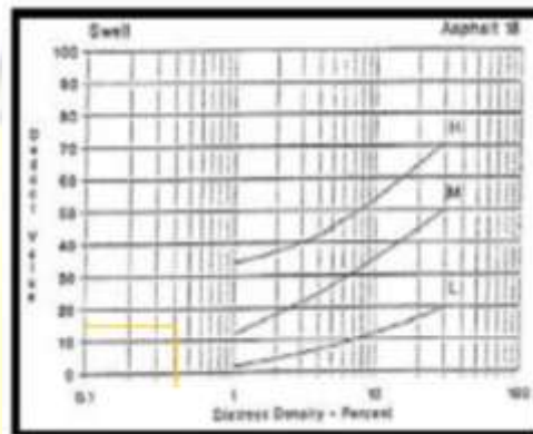
Gambar 2.36 Deduct value mengembang . (Sumber : Shahin, 1994)
