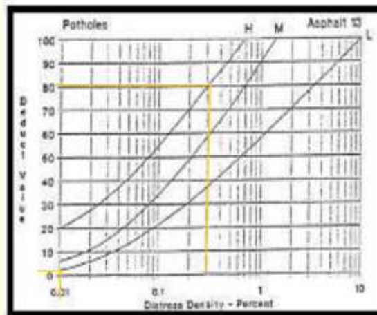
Gambar 2.34 Deduct value lubang. (Sumber : Shahin, 1994)
