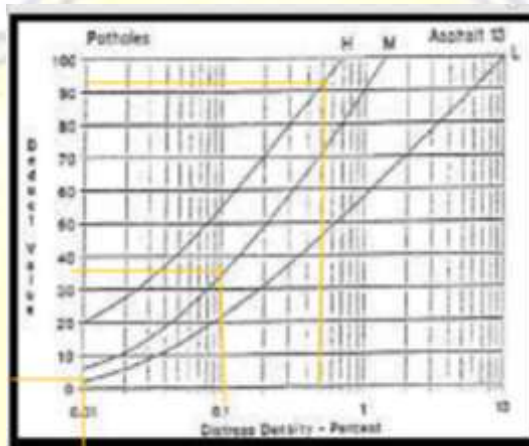
Gambar 2.34 Deduct value lubang. (Sumber : Shahin, 1994)
