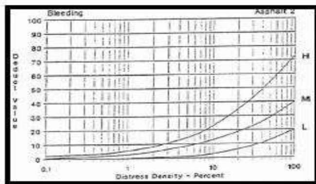
Gambar 2.24 Deduct value kegemukan. Sumber : Shahin, 1994
