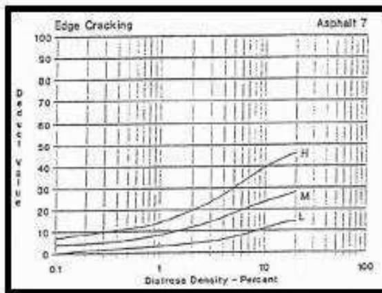
Gambar 2.28 Deduct value retak samping jalan. (Sumber : Shahin, 1994)
