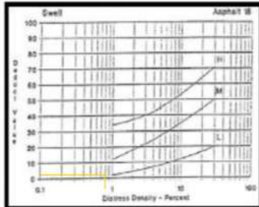
Gambar 2.36 Deduct value mengembang . (Sumber : Shahin, 1994)
