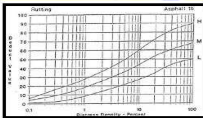
Gambar 2.40 Deduct value alur. (Sumber : Shahin, 1994)
