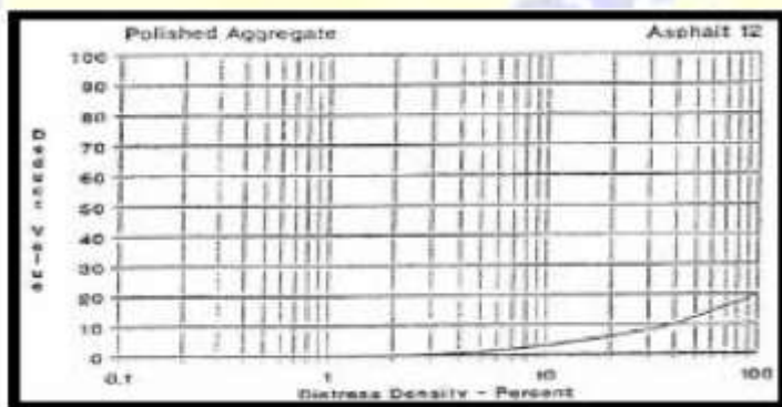
Gambar 2.34 Deduct value pengausan agregat. (Sumber : Shahin, 1994)
