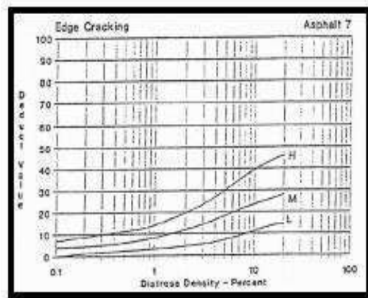
Gambar 2.28 Deduct value retak samping jalan. (Sumber : Shahin, 1994)
