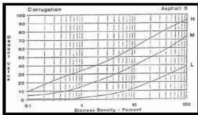
Gambar 2.27 Deduct value keriting. (Sumber : Shahin, 1994)
