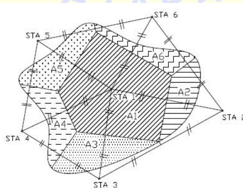
Gambar 2.1 Metode Polygon Thiessen
