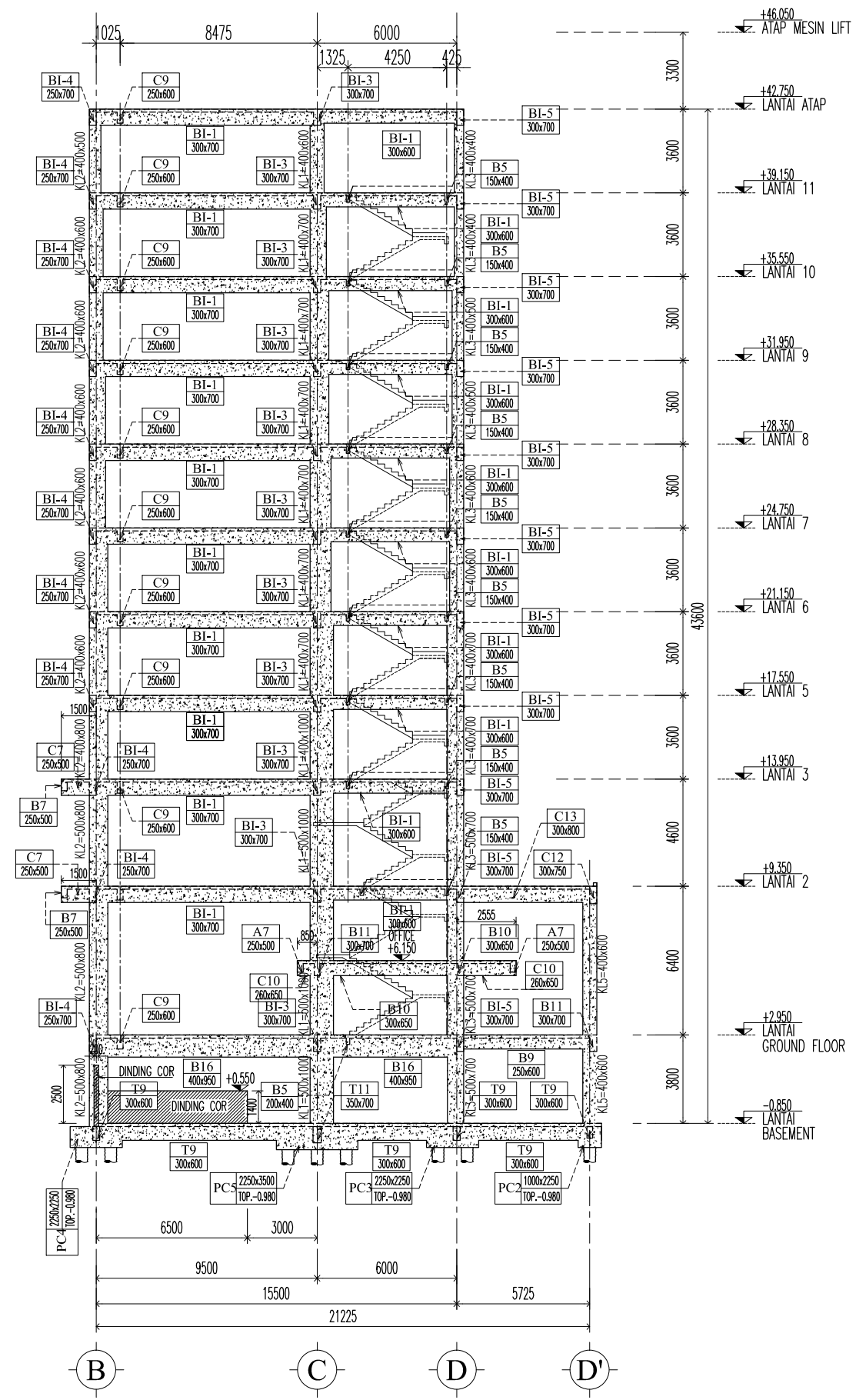
POTONGAN PORTAL T2 SKALA 1:250
